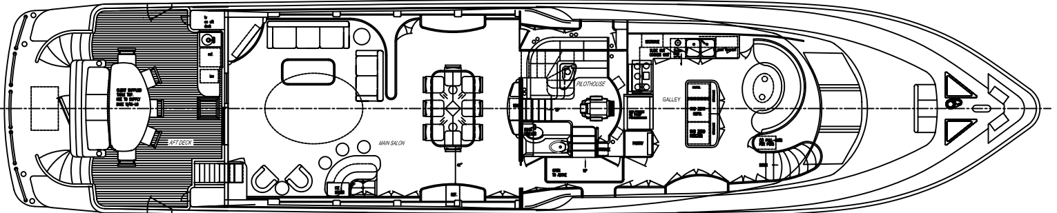
MAIN DECK
